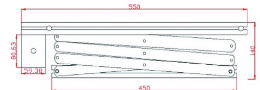
All dimensions are in mm
