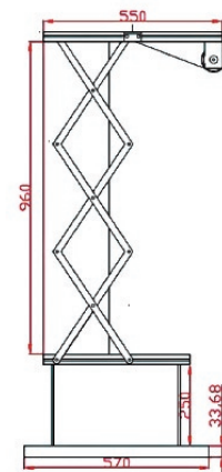
Lift lowered side view
