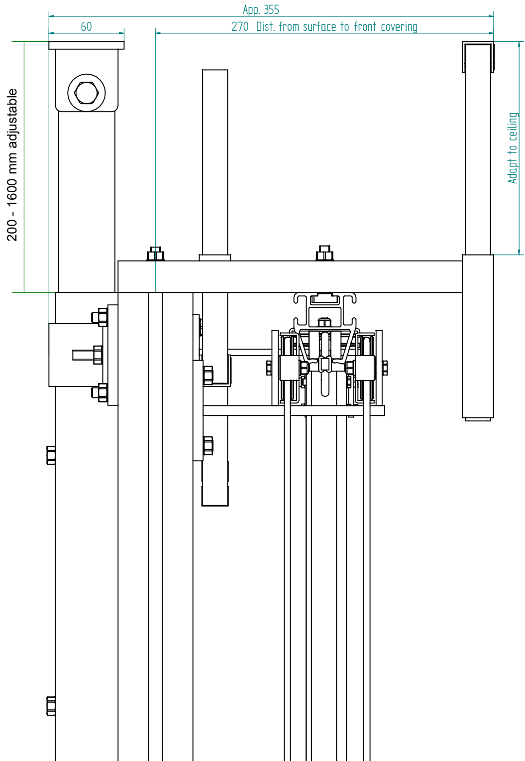
DETAIL K
